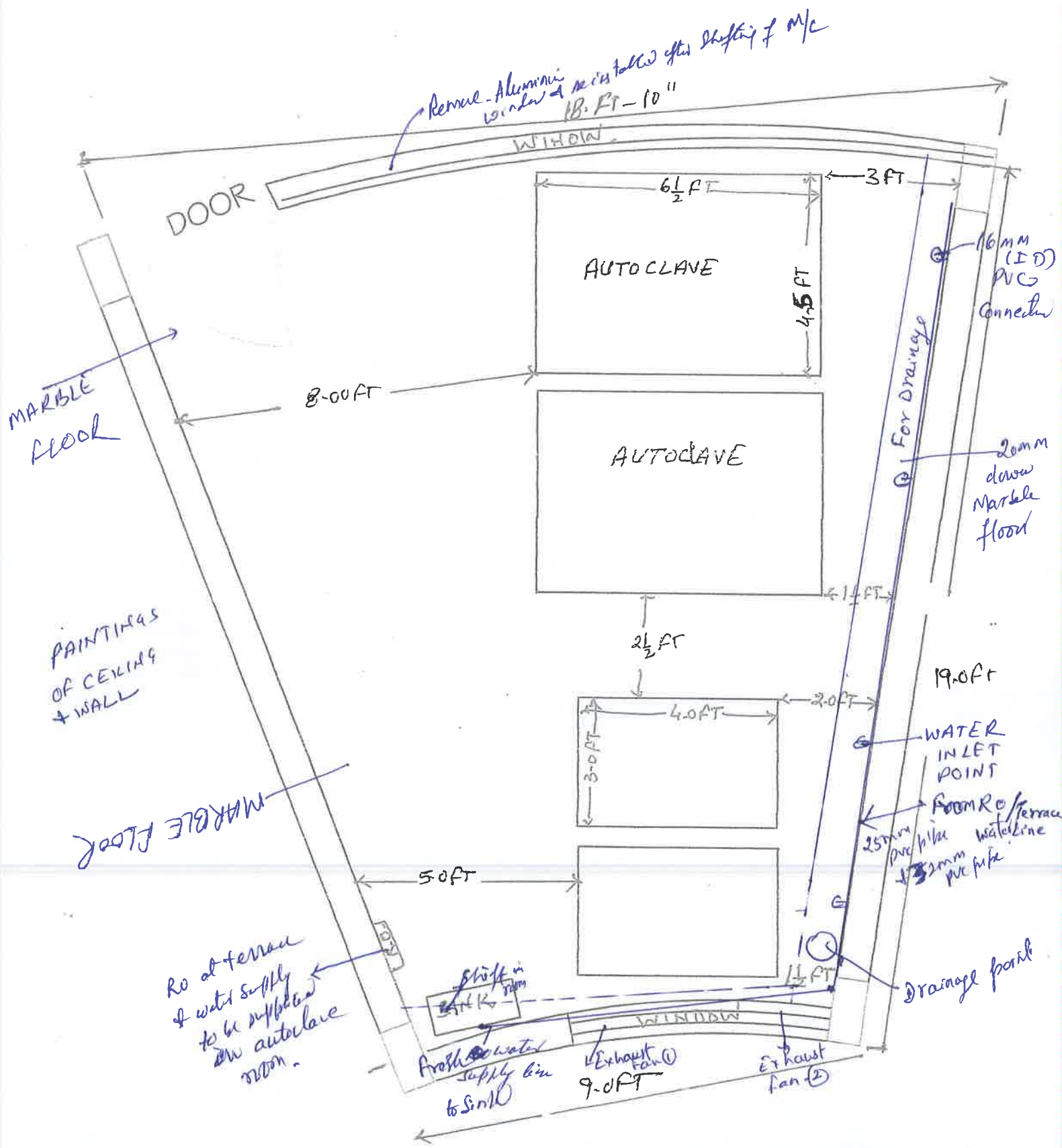
AUTOCLAVE ROOM
