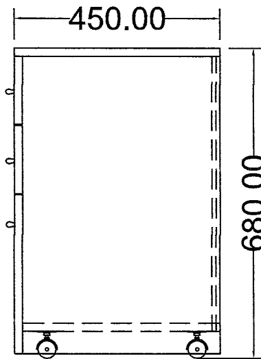
Side Elevation
