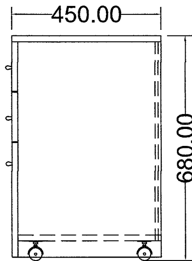
Side Elevation
